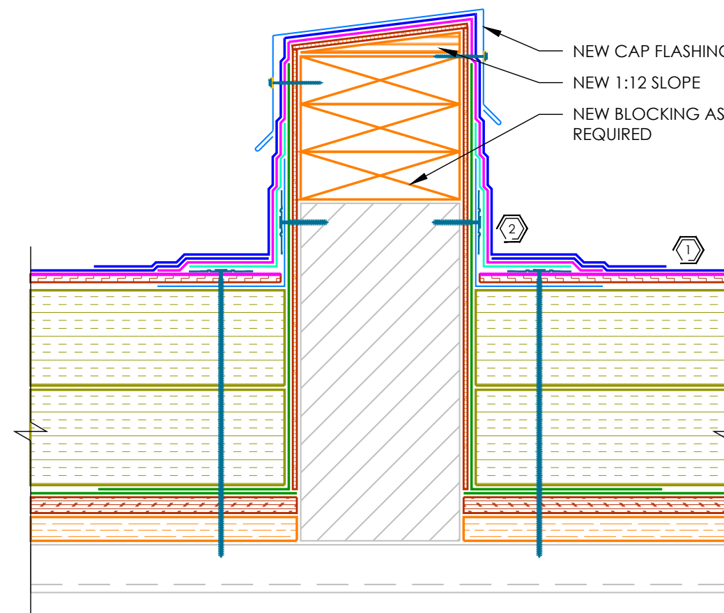
2 AREA DIVIDER NTS
